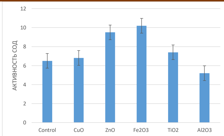
Fig. Effect of nanoparticles of biogenic metals on the activity of superoxide dismutase (in conditional units). Each bar represents mean \pm sd (standard deviation) for average of n=3 independent experiments; P = 0,05 .
